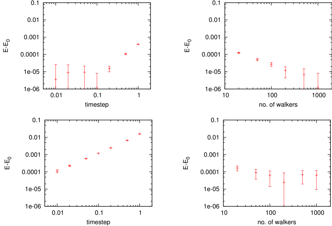
FIG. 4: (top-left) The convergence of the ground state energy with imaginary time step for the one-dimensional harmonic oscillator computed using the NC-DMC method with \psi_T = \psi_0(\lambda\omega) ; \lambda = 0.9 ; \epsilon \neq 0 and N = 1000 walkers. (top-right) The corresponding convergence of the ground state energy with walker number computed using an imaginary time step of \tau\hbar\omega = 0.1 . (bot-left) The convergence of the ground state energy with imaginary time step for the one-dimensional harmonic oscillator computed using the NC-DMC method with \psi_T = \psi_0(\lambda\omega) ; \lambda = 0.9 ; \epsilon = 0 and N = 1000 walkers. (bot-right) The corresponding convergence of the ground state energy with walker number computed using an imaginary time step of \tau\hbar\omega = 0.002 .
