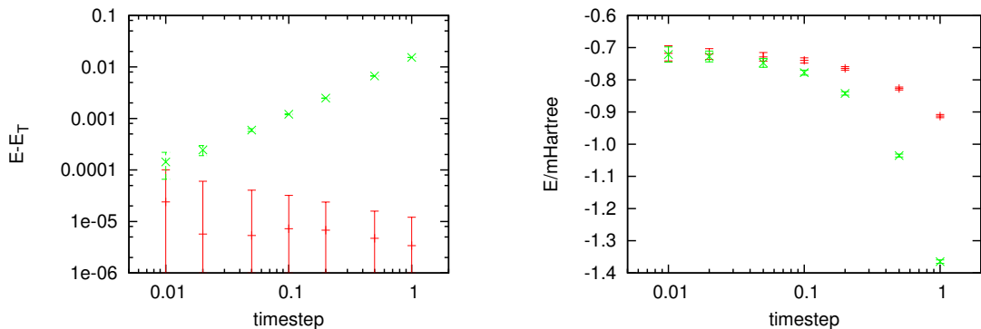
FIG. 11: (left) The convergence of the variational energy with imaginary time step both with and without the exact drift ( \epsilon \neq 0 , dash, and \epsilon \equiv 0 , cross), for the one-dimensional harmonic oscillator computing using the DMC method without branching and \psi_T = \psi_0(\lambda\omega) ; \lambda = 0.9 ; (right) The convergence of the variational energy with imaginary time step both with and without the exact drift ( \epsilon \neq 0 , dash, and \epsilon \equiv 0 , cross), for the full QDO xenon dimer computing using the DMC method without branching and the on-site-plus-all-pair-multipole trial function.
