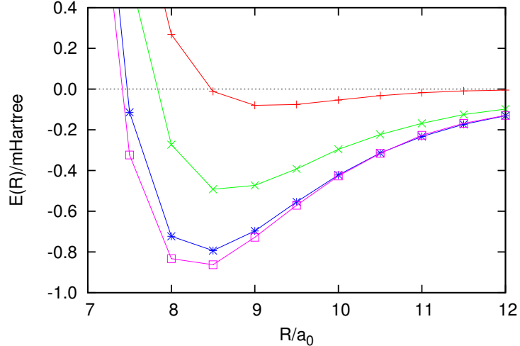
FIG. 5: The variational energy as a function of nuclear separation, E_T(R) for the full QDO model xenon dimer is presented for all trial wavefunctions described in the text, from top to bottom: The on-site-only trial function (plus sign), the on-site-plus-dipole-dipole trial function (x) and the on-site-plus-all-pair-multipole model (star). Results are compared to a converged NC-DMC study (box) of the dimer potential curve, E_0(R) .
