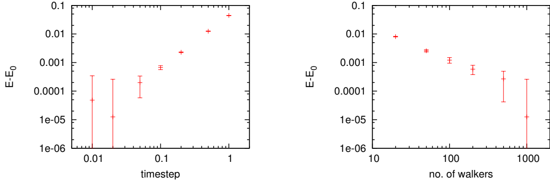
FIG. 3: (left) The convergence of the ground state energy with imaginary time step for the one-dimension harmonic oscillator computed using the NC-DMC method with \psi_T = 1 and N = 1000 walkers. (right) The corresponding convergence of the ground state energy with walker number computed using an imaginary time step of \tau\hbar\omega = 0.02 .
