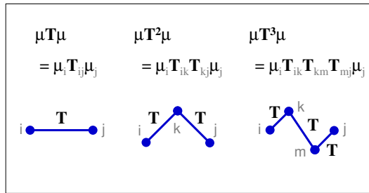
FIG. 1: Diagrams representing the leading contributions in the exponent of the trial wavefunction, see Eq. (34).
