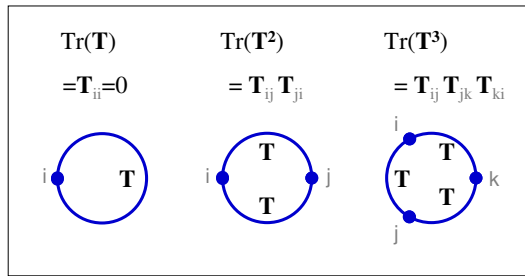
FIG. 2: Diagrams representing the leading contributions to the dipole-dipole interaction energy, as in Eq. (35c).
