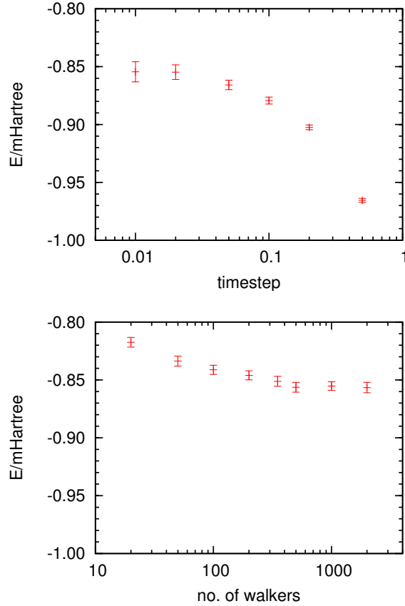
FIG. 6: (top)The convergence of the ground state energy with imaginary time step for the full QDO model xenon dimer computed using the NC-DMC method with the on-site-plus-all-pair-multipole trial function. (bot)The corresponding convergence of the ground state energy with walker number computed using an imaginary time step of \hbar\tau = 0.02\text{au} . Note, the energy scale is on order 10\mu\text{Hartree} , stringently testing the method.
