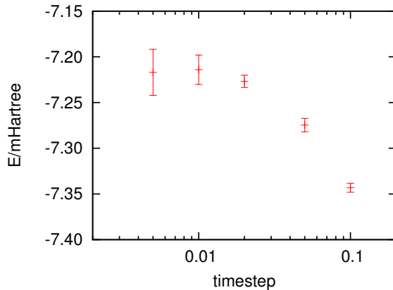
FIG. 8: The convergence of the ground state energy of the fcc-xenon solid as a function of imaginary time step at the equilibrium lattice constant under the full QDO model computed using NC-DMC with the on-site-plus-all-pair-multipole trial function, with 32 atoms and N = 1000 walkers.
