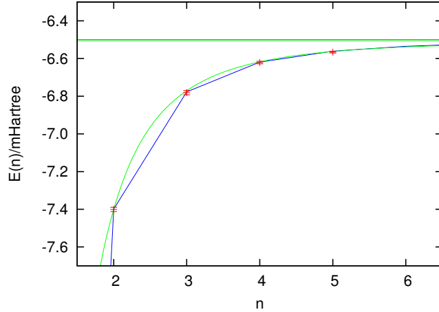
FIG. 7: The convergence of the ground state energy of the fcc-xenon solid at the equilibrium lattice constant as a function of system size ( n = n_{cell} ) under the dipole limit QDO model computed using NC-DMC with the on-site-plus-dipole-dipole trial function, N = 1000 walkers and a time step of \hbar\tau = 0.01 . Simulation results (points) are compared to the analytical results (blue). A fit to the data is included ( f(n) = E_0 - \Delta/n^3 ) along with the extrapolated value of E_0 = -6.5055 mHartree/atom (top horizontal line), which is close to the large- N analytic result of E_0 = -6.4996 mHartree/atom, calculated for N = 32000 (purple).
