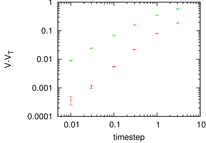
FIG. 12: (left) The convergence of V_T = -\langle e^2/r \rangle_{\psi_T^2} = (-e^2/a_0) for the hydrogen atom, \psi_T = \exp(-r/a_0) , with imaginary time step both with and without the isotropic diagonal approximation to the trial function 2nd derivative matrix ( \epsilon = -2\hbar^2/(3mra_0) , dash, and \epsilon \equiv 0 , cross) computed using the DMC method without branching in Cartesian coordinates.
