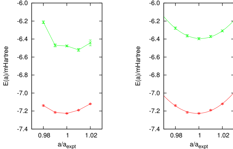
FIG. 10: (left) The ground state energy of the M_{Xe}=32 atom fcc-xenon solid as a function of lattice constant, E_0(a) under the full QDO model computed using NC-DMC with the on-site-plus-all-pair-multipole trial function (bottom curve), N = 1000 walkers and an imaginary time step of \hbar\tau = 0.02\text{au} . compared to the variational result of the on-site-plus-all-pair-multipole trial function (top curve). (right) The ground state energy of fcc-xenon for M_{Xe}=32 atom (bottom curve) and M_{Xe}=256 atom (top curve) cells solid as a function of lattice constant, E_0(a) , under the full QDO model computed using NC-DMC with the on-site-plus-all-pair-multipole trial function, N = 1000 walkers and an imaginary time step of \hbar\tau = 0.02\text{au} .
