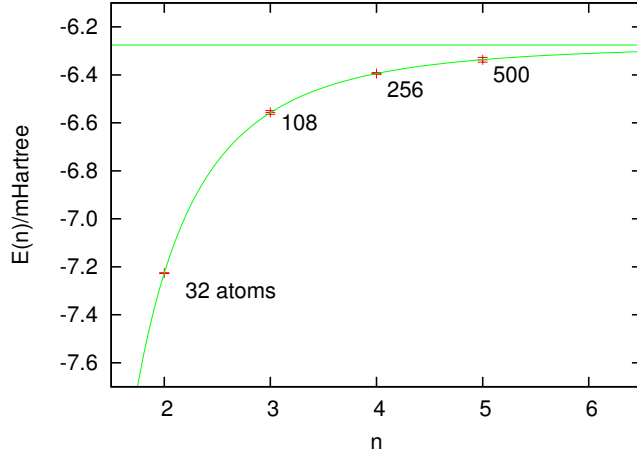
FIG. 9: The convergence of the ground state energy of the fcc-xenon solid as a function of system size ( n = n_{cell} ) at the equilibrium lattice constant under the full QDO model computed using NC-DMC with the on-site-plus-all-pair-multipole trial function (the points), N = 1000 walkers and an imaginary time step of \hbar\tau = 0.02\text{au} . A fit to the data is included ( f(n) = E_0 - \Delta/n^3 ) along with the extrapolated value of E_0 = -6.275\text{mHartree/atom} (top horizontal line).
